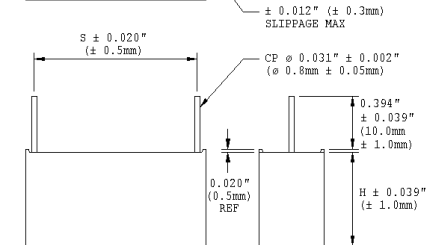
Terminal style 8 (TCW wire) Maximum case size 0.866"x1.378"x2.283" (22mmx35mmx58mm)
